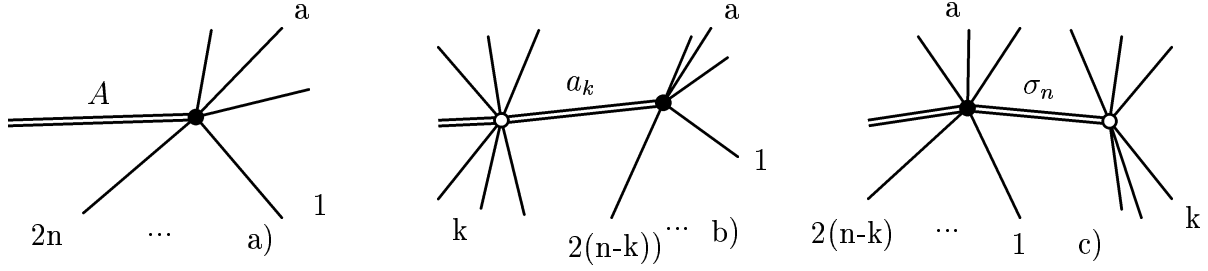
Figure 1: Contribution to decay A \rightarrow a + 2n\pi matrix element: a) without PV excitation, b) 2k pions created through PV excitation with quantum numbers of A intermediate state. c) 2k -pions created by PV excitation with vacuum quantum numbers intermediate state.
