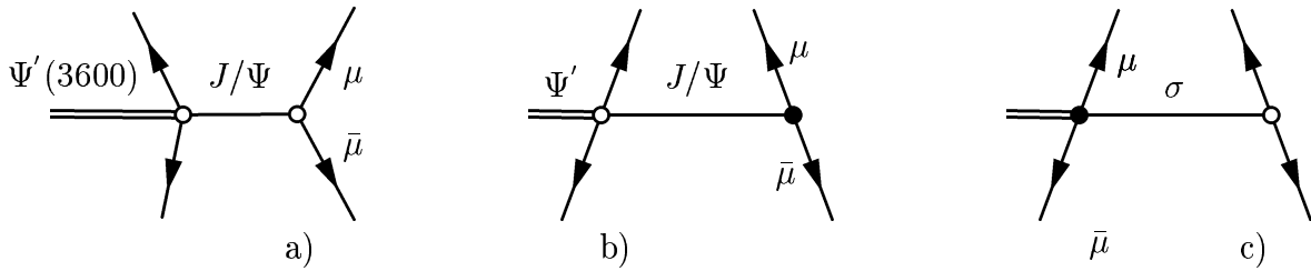
Figure 3: Feynman diagrams for \Psi'(3600) \rightarrow 2\pi\mu^+\mu^- decay: a) without PV excitation, b,c) two-pion created from PV excitation.
