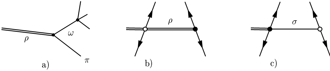
Figure 2: Feynman diagrams for \rho \rightarrow 4\pi decay: a) without PV excitation, b,c) two-pion production through PV excitation.
